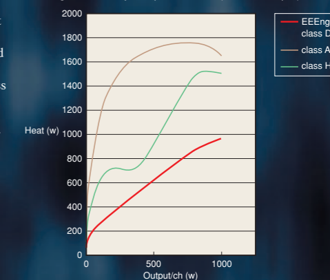
Fig.6. Efficiency comparison data (heat vs. output)
